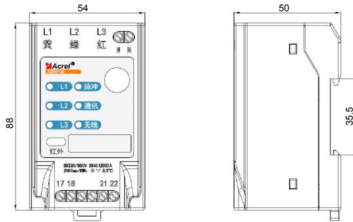
Fig 1 Dimension of AEW100
